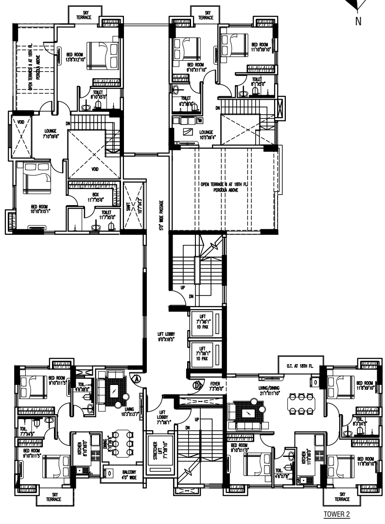
18TH FLOOR PLAN
